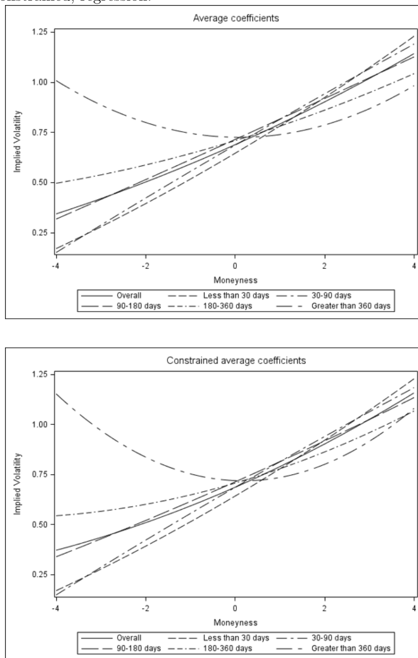
Figure 8: IV curves from mean coefficients. This figure shows the IV curves predicted by the mean factors (level, slope and curvature) for different maturity categories. The top plot shows this for the unconstrained while the bottom plot shows it for the constrained, regression.
