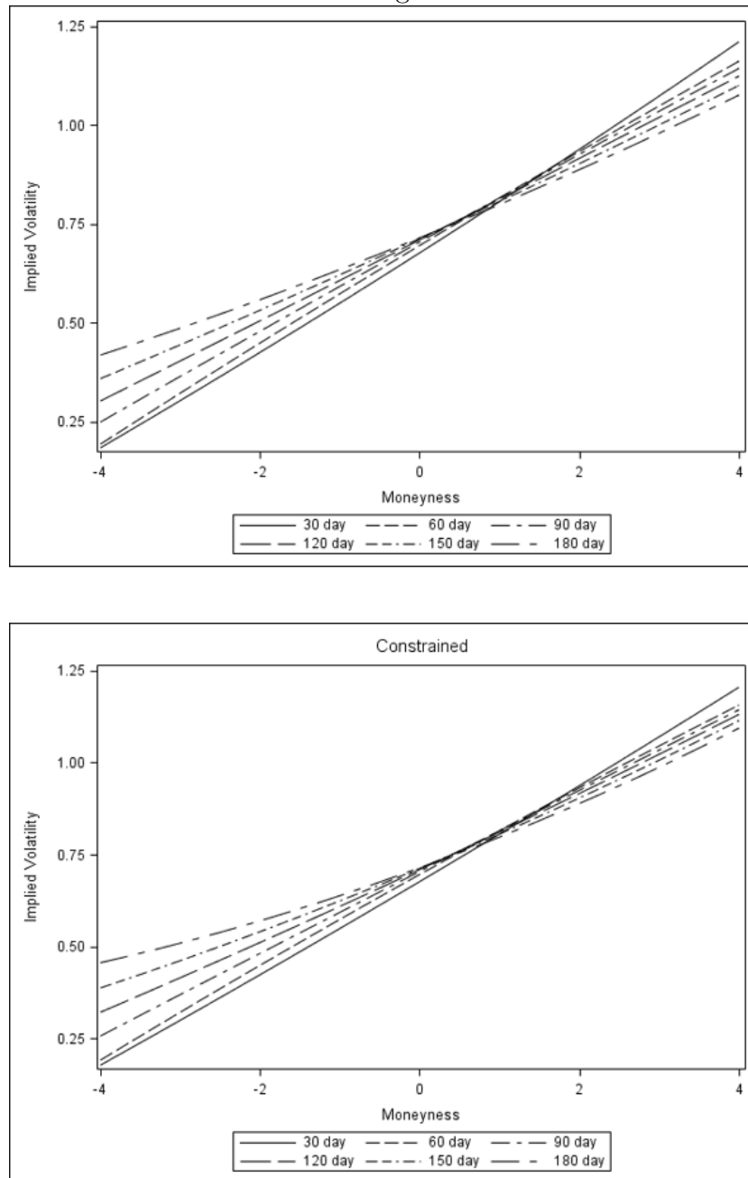
Figure 13: IV curves from mean interpolated coefficients. This figure shows the IV curves predicted by the mean interpolated factors (level, slope and curvature) for different maturities. The top plot shows this for the unconstrained while the bottom plot shows it for the constrained regression.
